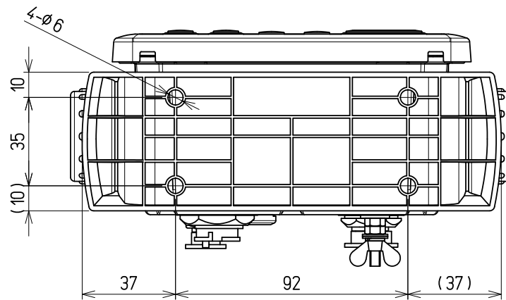
Mount (bottom)
