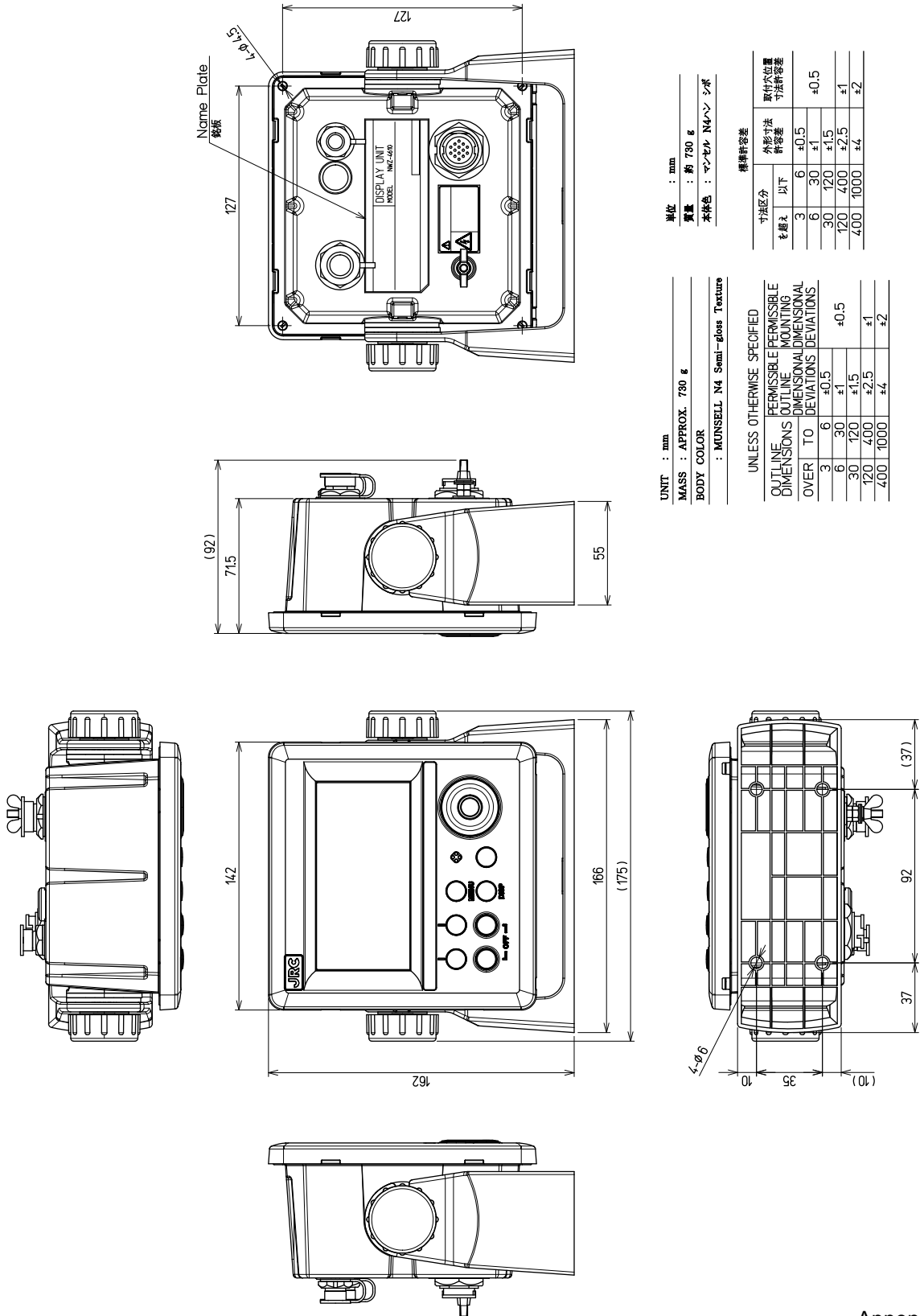
(1) NWZ-4610 MAIN DISPLAY (Desk form type)
