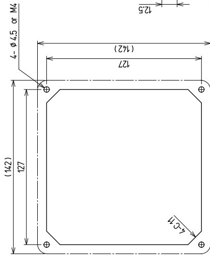
取付穴寸法図 SETTING HOLES DRAWING
