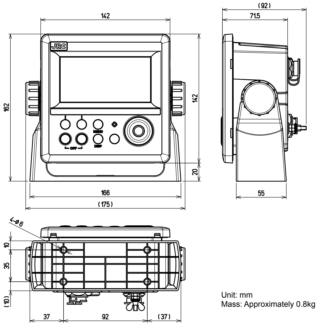
Figure 1.2 NWZ-4610 OUT LINE (Disk Form type)
