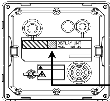
Display Unit Rear
