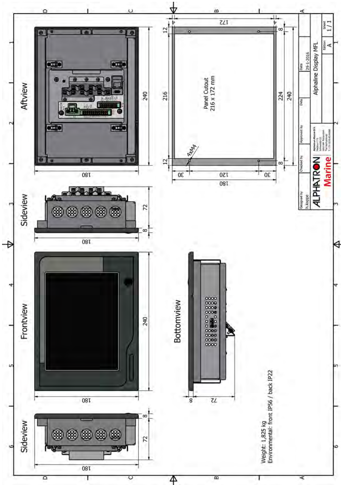
Figure 45: Mechanical Drawing MFL
