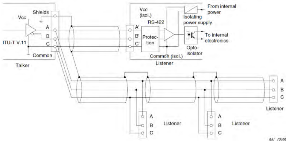
Figure 8: IEC 61162-2 Circuits
