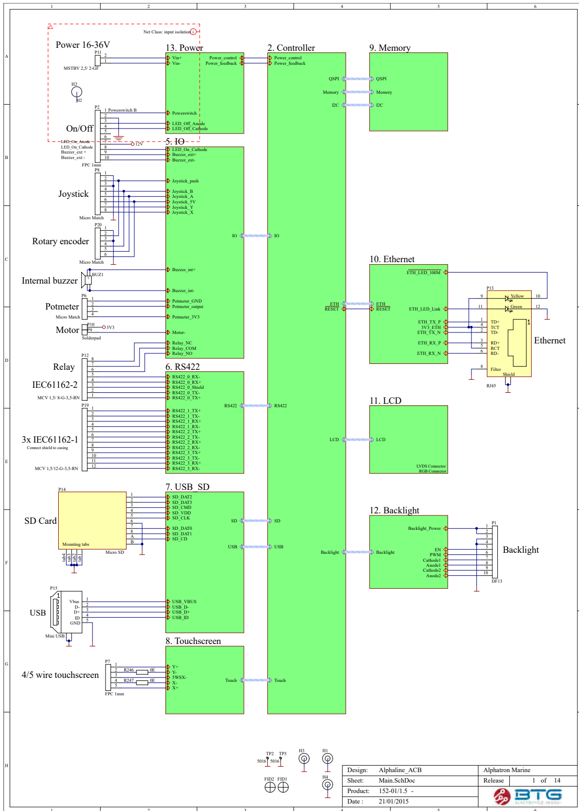
Figure 49: Schematics AlphaLine Instrument
