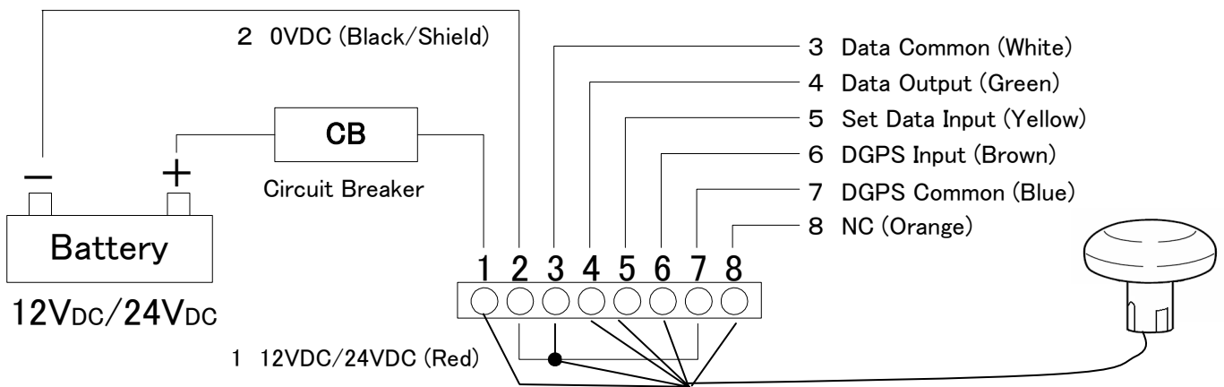
Fig. 3-3 Indirectly connectable Navigation Equipment
